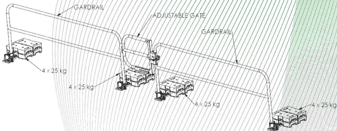
Figure 1: edge protection system type: Guard Trac
